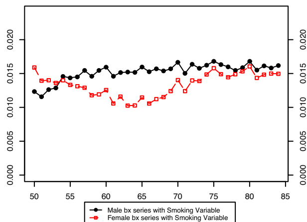
Fig. 4. Comparison of male and female b_x values in a model with smoking histories: United States, 1969-2003.
